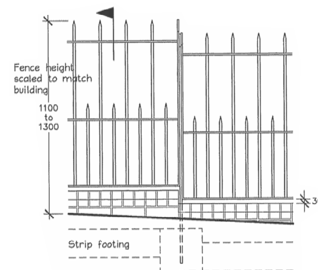
FENCE WITH STEPPED PLINTH For sloping sites
