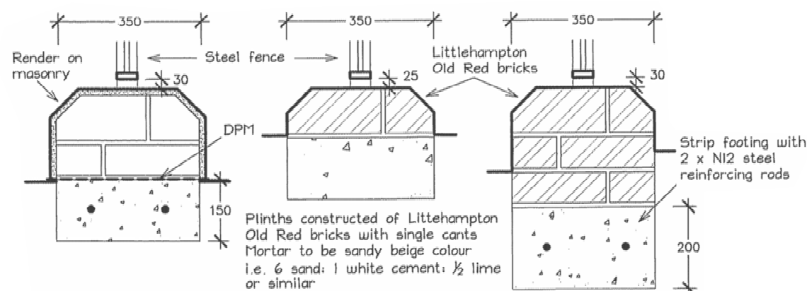
RENDERED PLINTH For flat sites
